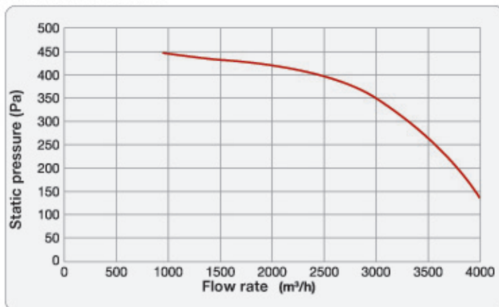
BD 10/10 4P 0.59 kW
